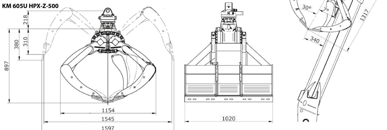
KM 605U HPX-Z-500
